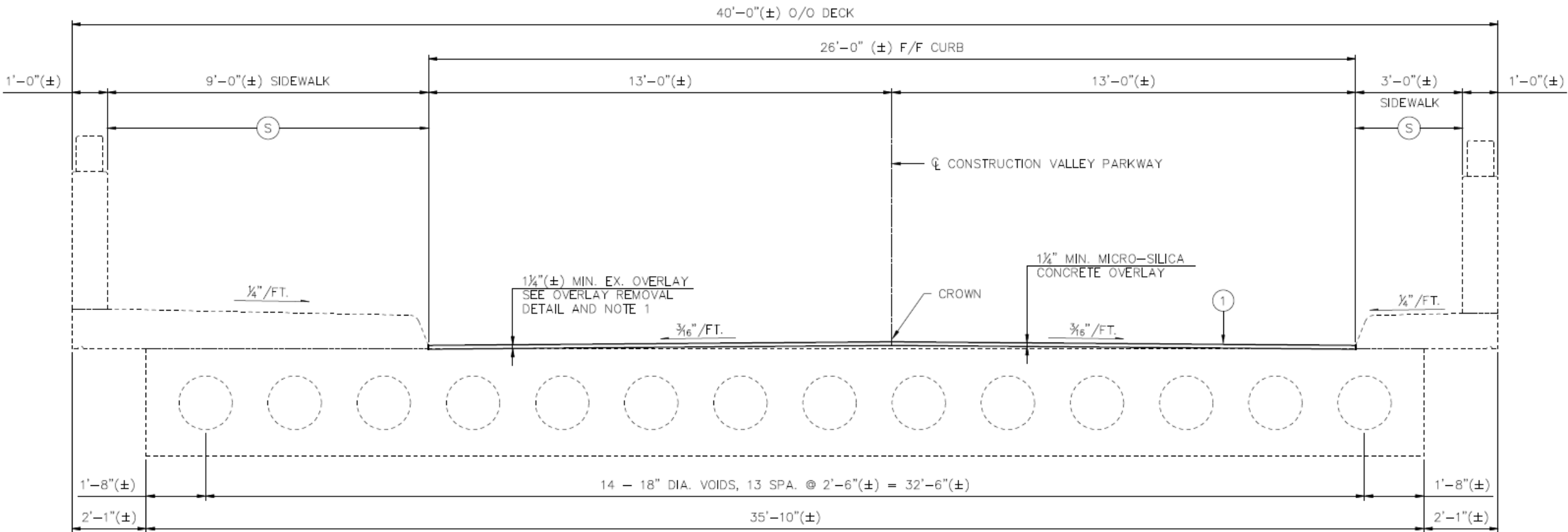
TRANSVERSE SECTION
