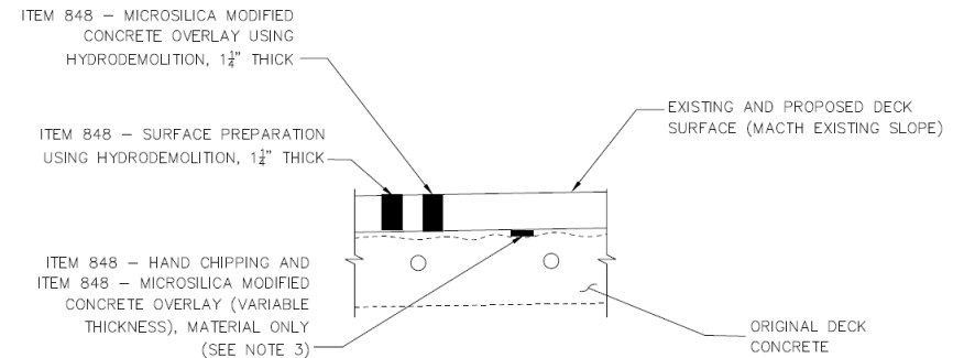
BRIDGE DECK WEARING SURFACE REPLACEMENT DETAIL
