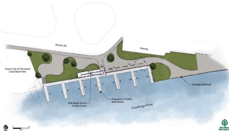
HERITAGE PARK 1 - Boat Dock Plan
